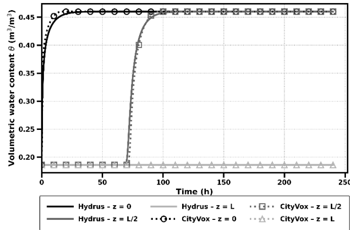
Figure 1: Time evolution of volumetric water content \theta at three depths (surface, mid-depth, and bottom) simulated by Hydrus-1D and the CityVox water module.
