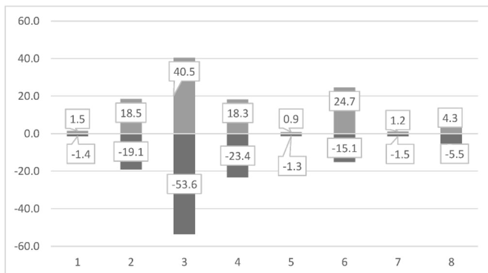
Figure 6: Sensitivity Study - Parameter Variations vs. System Mass flow rate (% change)
