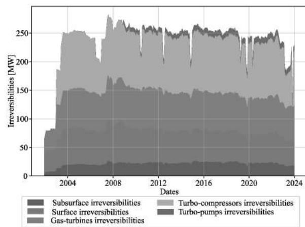
Figure 5 : Irreversibilities simulation
