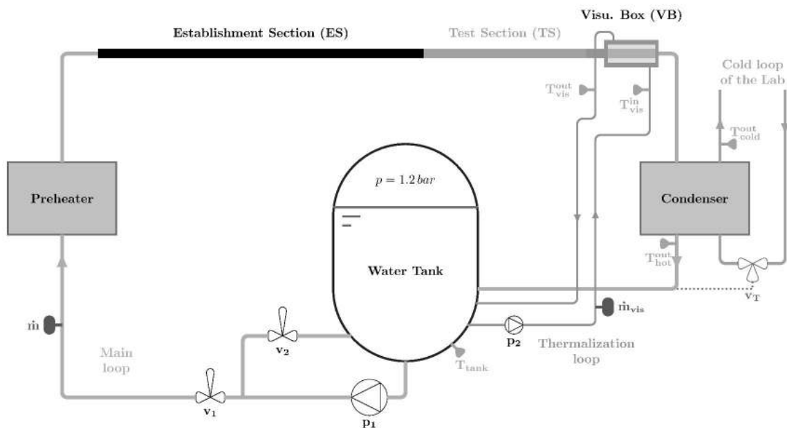
Figure 1 : Schematic layout of the ConBo experimental facility.
