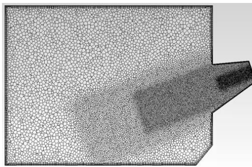
Figure 4 : Maillage cas plasma
