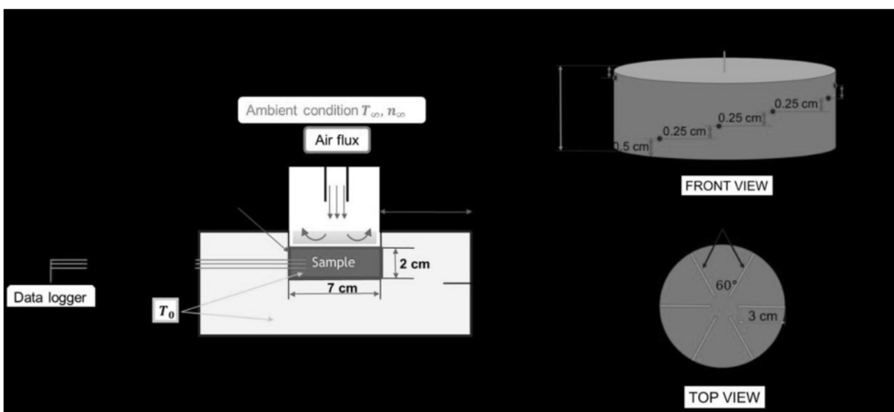
Fig. 2. a) The experimental setup of heat and mass transfer; b) the arrangement of the thermocouples.
