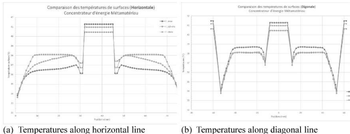
Figure 9: Temperature distributions along horizontal and diagonal lines for the different tested configurations of thermal concentrators
