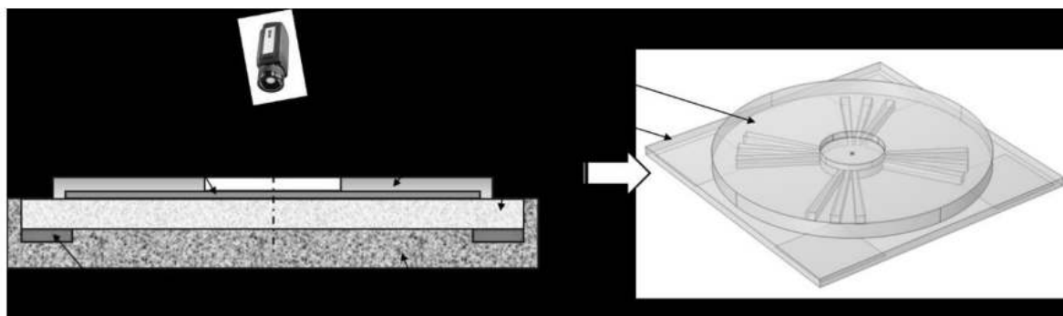
Figure 1: Presentation of the different elements of the experimental setup.
