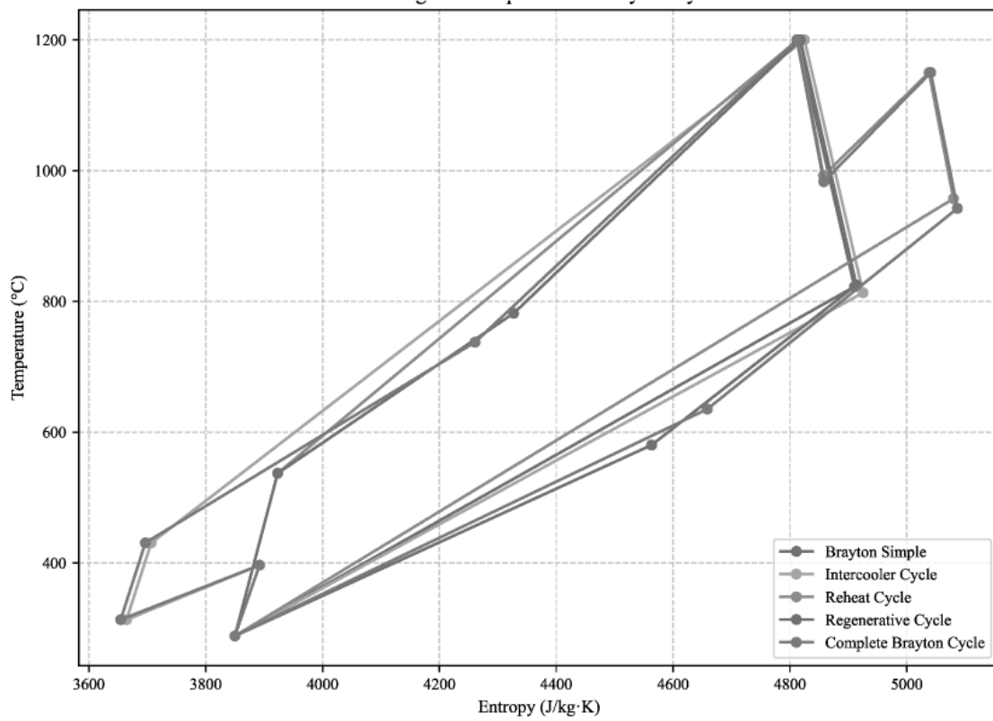
Figure 2 : Temperature-Entropy diagram comparing the five Brayton cycle configurations. All parameters are set to their reference values given in Table 2.
