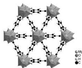
Figure 3 : Structure cristalline du MOF Mg(H_2gal) ( H_4gal = acide gallique)
