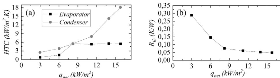
FIGURE 5 – (a) HTC of the evaporator and condenser, (b) thermal resistance of the system.
