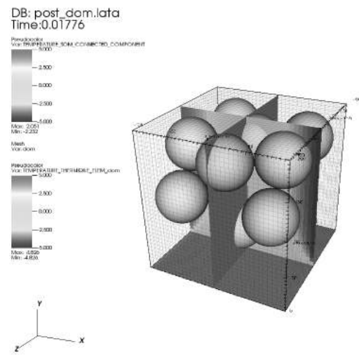
(b) Temperature convergence of particles initially at 0 °C with walls temperatures at \pm 5 °C gradient.
