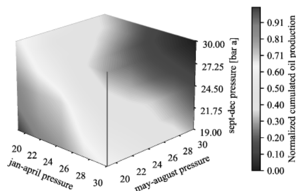
Figure 7 : Cumulated oil influence pressure
