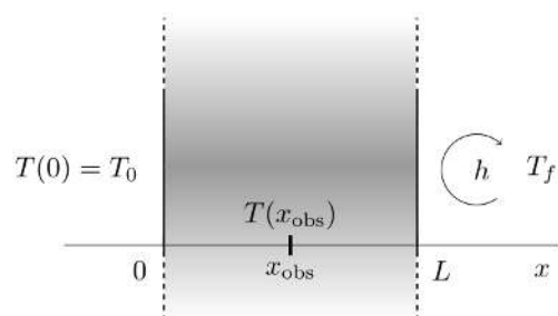
Figure 1 : 1D steady-state conduction-convection configuration.
