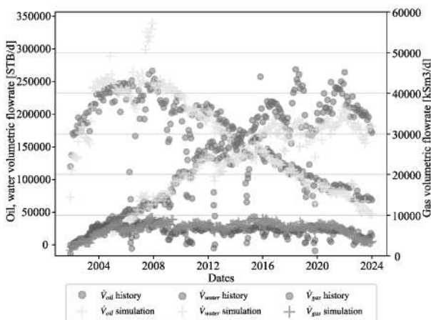
Figure 4 : Oil, gas & water production history match
