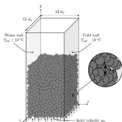
Figure 3 : Configuration of the fluidized-bed simulations.
