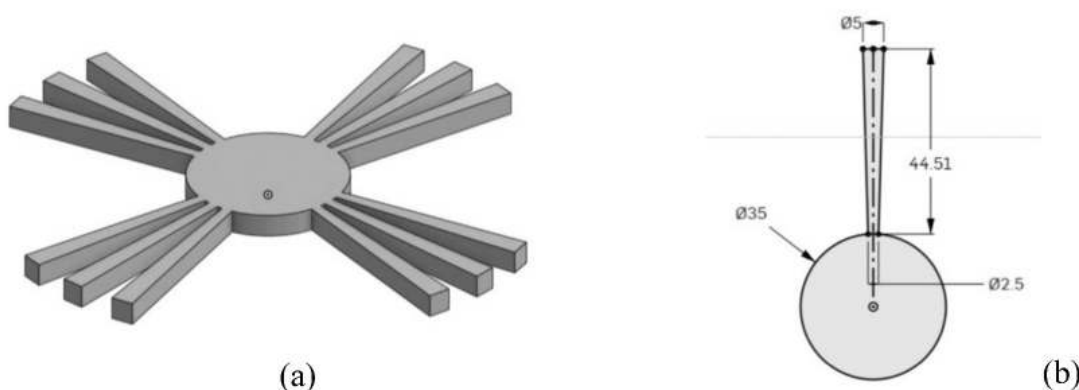
Figure 2: Presentation of the central part of the copper concentrator (a) and its dimensions (b).
