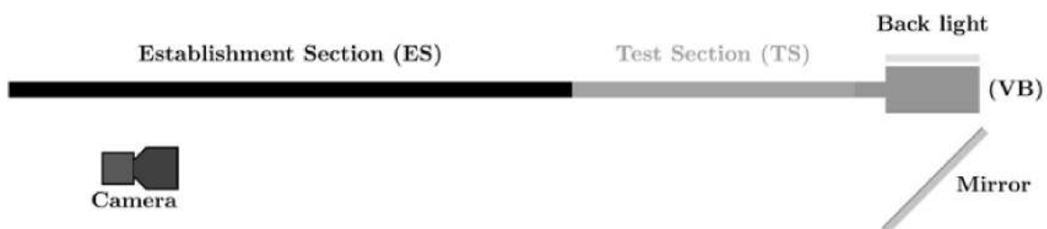
Figure 2 : Top view scheme of the optical setup.
