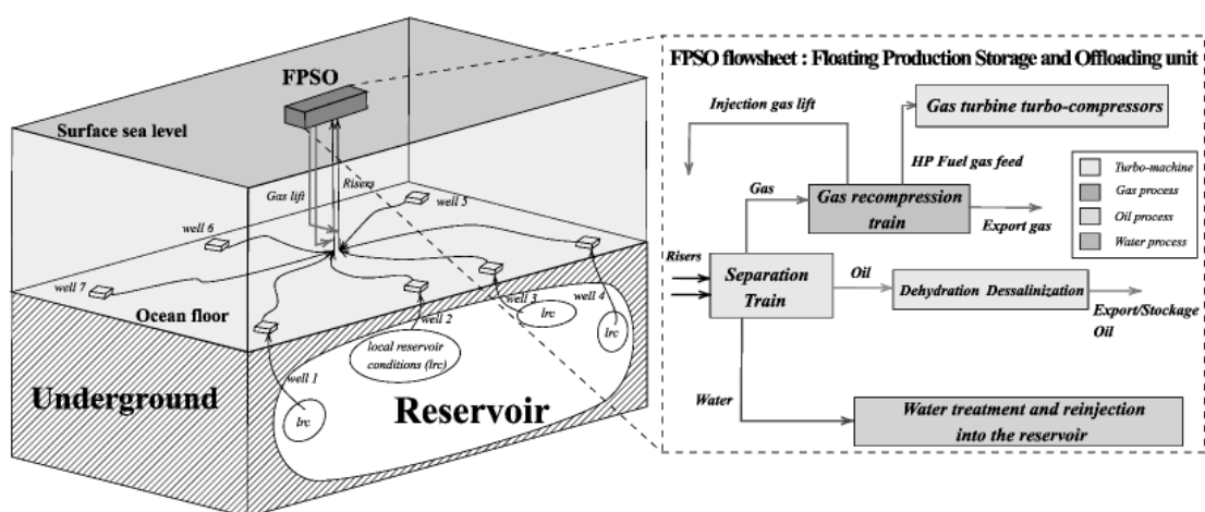
Figure 1 : Girassol field flowsheet
