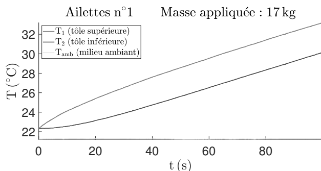
Figure 6 : Thermogrammes
