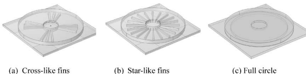
Figure 8: Different tested configurations of thermal concentrators
