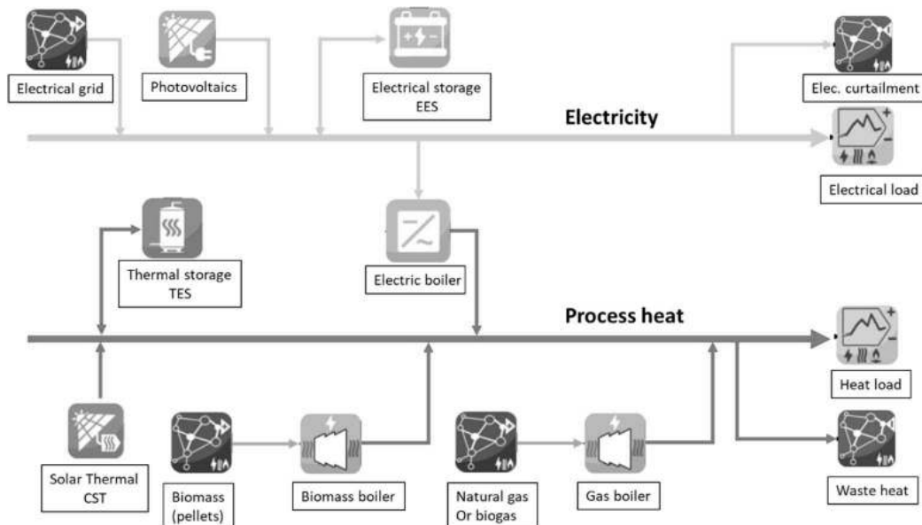
Figure 1 : Hybrid energy system architecture.
