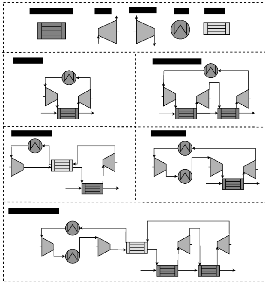
Figure 1 : Illustration of the 5 Brayton cycle configurations studied.
