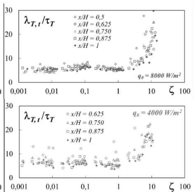
Figure 10 : Micro-échelle temporelle turb. therm.
