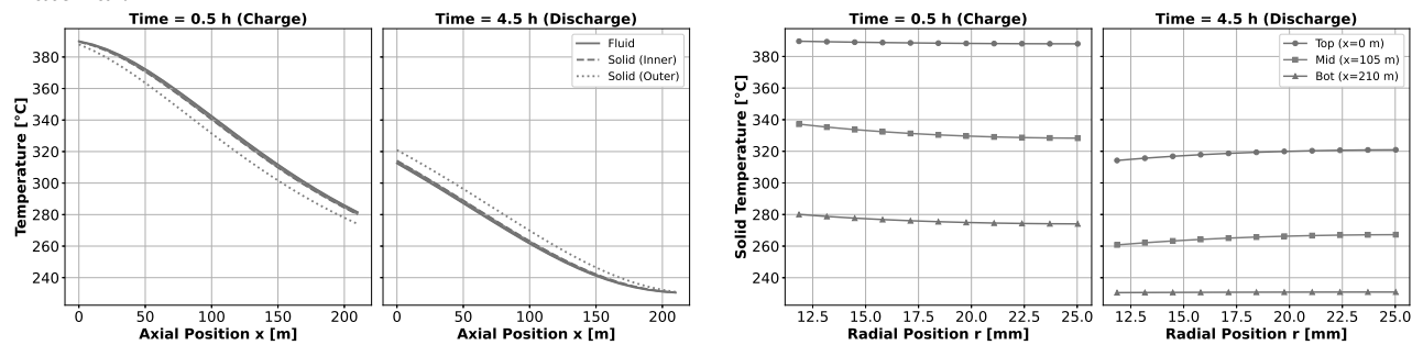
(a) Axial fluid and solid temperature profiles
