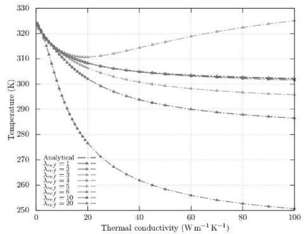
Figure 5 : Temperature estimates T(x_{\text{obs}}, \lambda) for \lambda \in [0, 100] and different \lambda_{\text{ref}} . x_{\text{obs}} = L/2 , T_f = 350 K, T_0 = 300 K.
