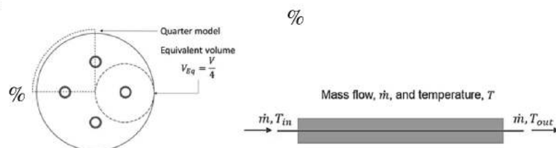
Figure 3: Assumed long tube and quarter model derived from [4].
