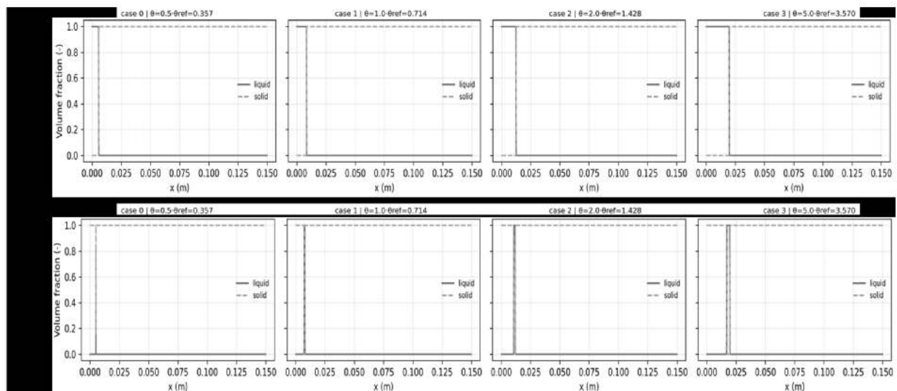
Figure 5 : Spatial distributions of solid and liquid volume fractions during (a) charging ( t = 10.5 h) and (b) discharging ( t = 13.8 h) phases for different values of \theta .
