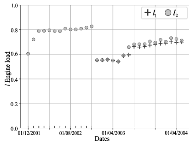
Figure 9 : I optimization results
