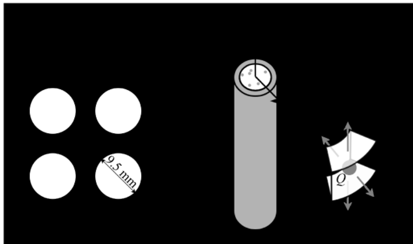
Figure 1 : Schematic drawing of the subchannel geometry (left) and the heat conduction problem (right)
