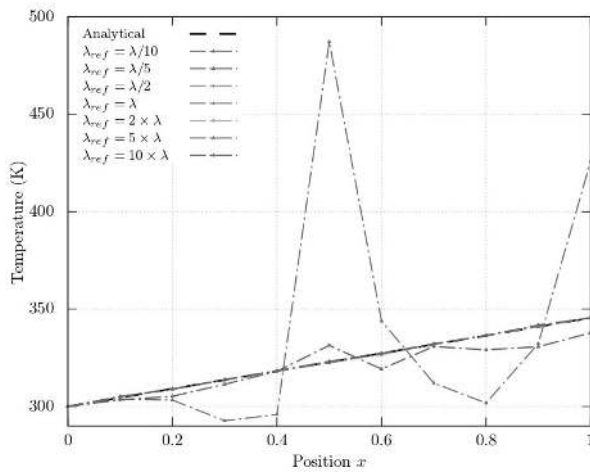
Figure 4 : Analytical vs. SMC results for \lambda = 1 and various \lambda_{\text{ref}} .
