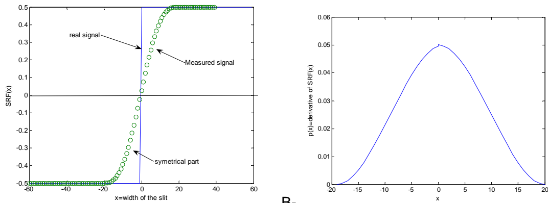
A- Figure 3: A-Example of Slit Response Function and corresponding pixel positions, B- Derivative of the previous SRF function: p(x) which is the kernel of the moving average applied to the signal.
