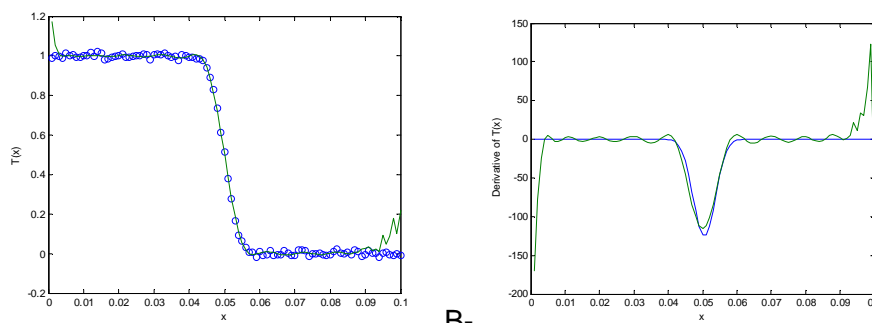
A- Figure 6: A-polynomial fitting of the signal shown on figure 5. B- Derivation.
