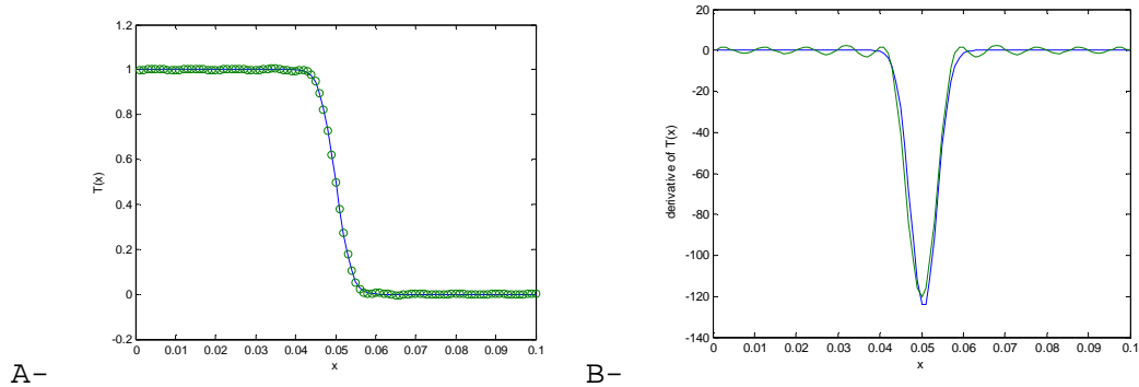
Figure 7: A-Fourier fitting of the signal shown on figure 5. B- Derivation. The number of terms is N=30 . The number of observation points is 100.
