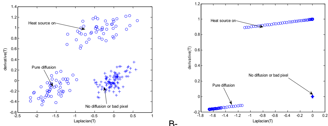
A- Figure 15 Study of the correlation between Laplacian and time derivative for several pixels ('o' pixel with or without source term with diffusion, '+' pixel where no diffusion appear or "bad pixel"). A- From noisy signal, B-From less noisy signal.
