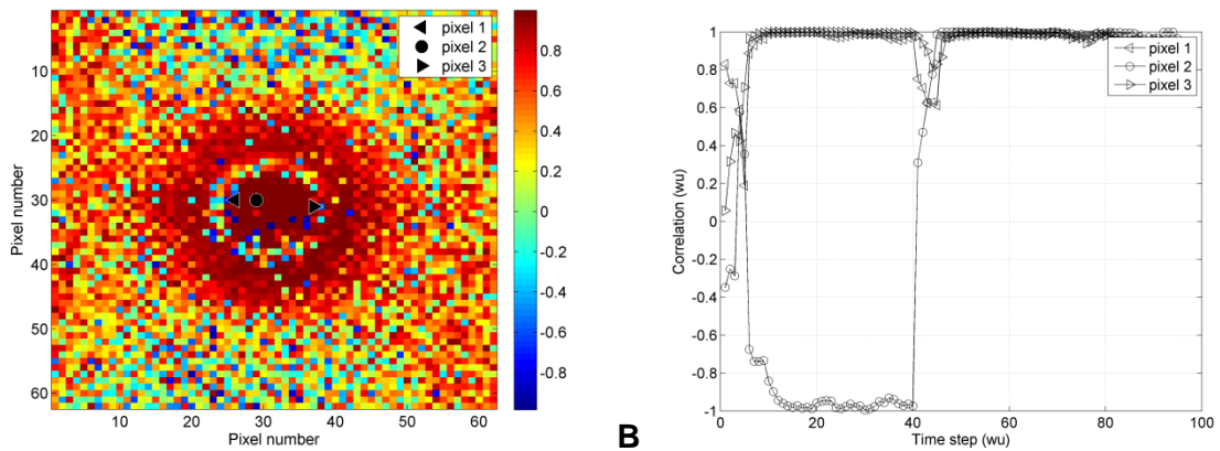
Figure.13 Correlation coefficients calculated for Ft = 4 . A- Field at t = 55 wu (just after the heat step) B- Time-evolution for 3 pixels at the center of the image.
