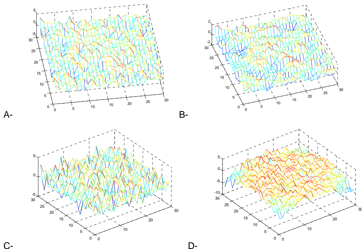
Figure 2; Examples of noise occurring with a 2D array of sensors, A- random Gaussian, B- non-isotropic spatial correlation, C- Digitized noise D-Non-uniformity distortion
