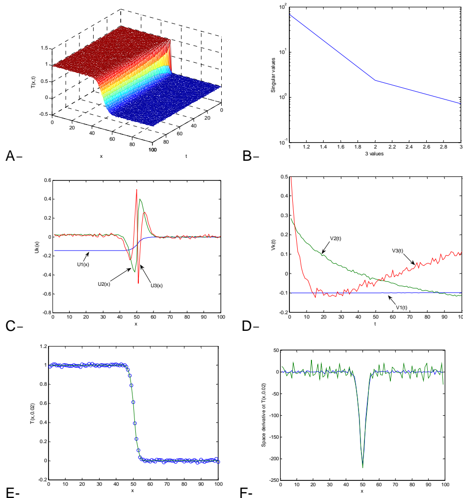
Figure 9: A- T(x,t) noisy temperature field (time extension from figure 5), B-3 first singular values,C-D-First \mathbf{U} and \mathbf{V} vectors, coming from the SVD decomposition, E- Reconstruction of the previous signal at time t=0.02 s, with 3 term of the SVD decomposition.F- “Noisy” derivation of the previous signal (initial noisy observation) compared the finite differences derivative of the SVD reconstruction)
