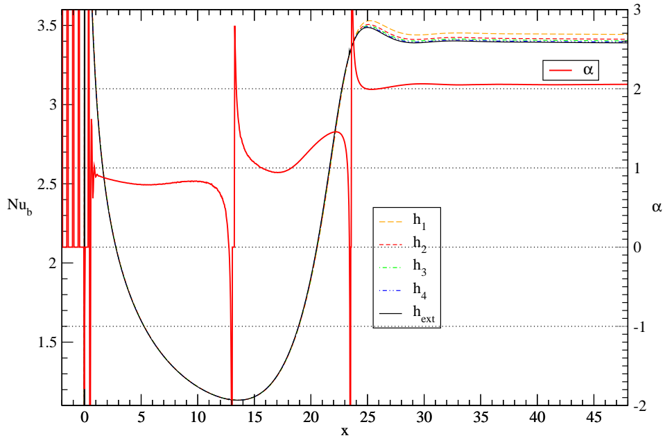
(a) Streamwise Nu profiles along (y, z) = (5, 0)
