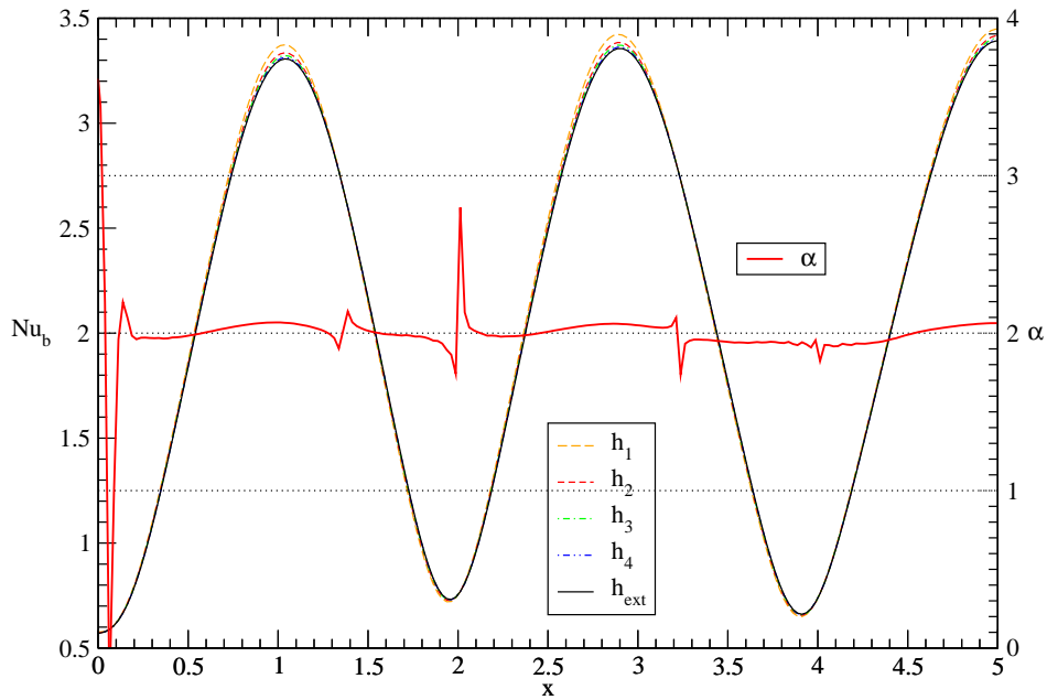
(b) Spanwise Nu profiles along (x, y) = (30, 0)
